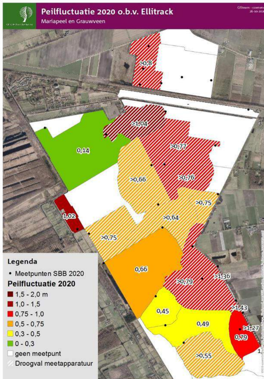
Figuur 3.10: Peilfluctuaties in Mariageel.
